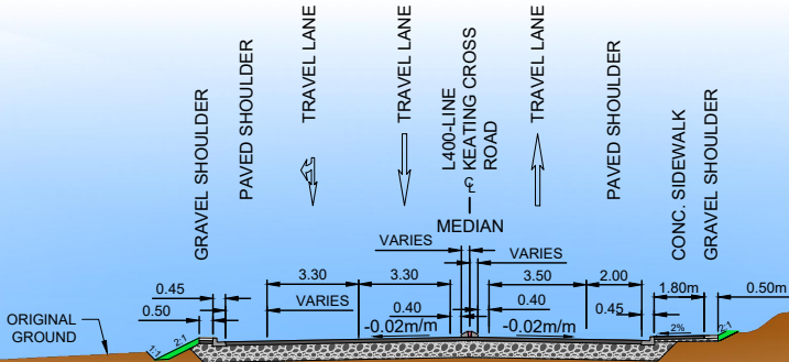
KEATING CROSS ROAD DISTRICT OF CENTRAL SAANICH PROPOSED - TYPICAL SECTION
