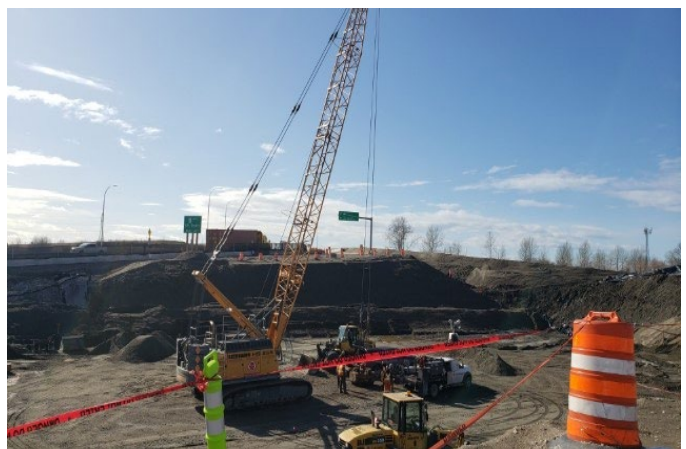
S1 River Rd structure – Stone Columns Installation nearing completion. Taken February 25, 2021
