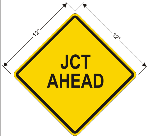
JUNCTION AHEAD Informs riders that they are approaching a trail intersection. 12 in. x 12 in. diamond. Yellow background, black lettering. Arial Bold Narrow 190 point character spacing 0% line spacing 85% character height.
