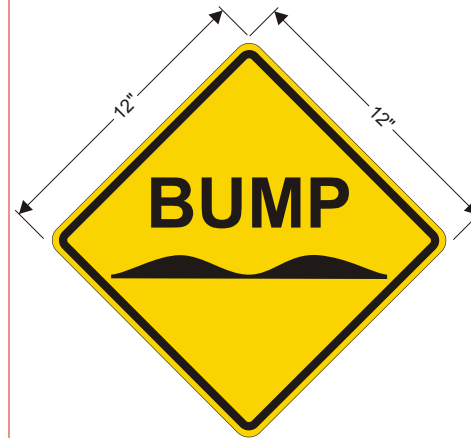
BUMP Informs riders that they are approaching a spot that is abruptly higher or lower than the trail on both sides. 12 in. x 12 in. diamond. Yellow background, black lettering. Arial Bold 210 point character spacing 0% line spacing 100% character height 11.5 x 1 in. black graphic.
