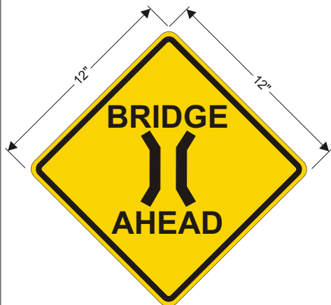
BRIDGE AHEAD Informs riders that they are approaching a bridge which is narrower than the trail. 12 in. x 12 in. diamond. Yellow background, black lettering. Arial Bold 135 point character spacing 0%. 4.5 x 3.25 in. black graphic.
