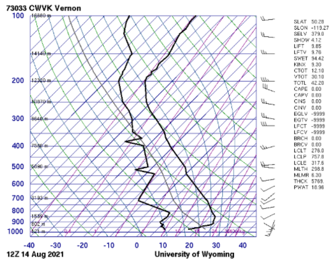
Figure 8. Temperature inversion at 0700 PDT
