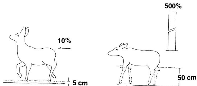
Figure 1. Relative increase in energy expenditure for movement of an adult deer through snow as compared to movement with no snow based on data from Parker et al. 1984.
