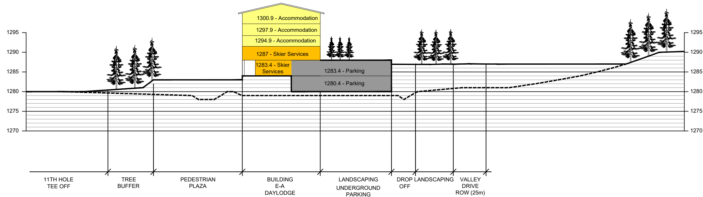
SECTION A'-A'
