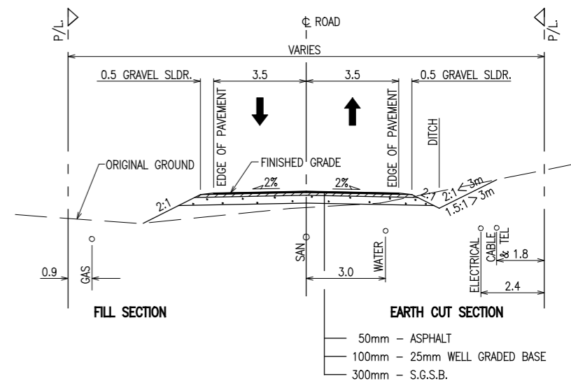
COLLECTOR ROAD TYPICAL SECTION
