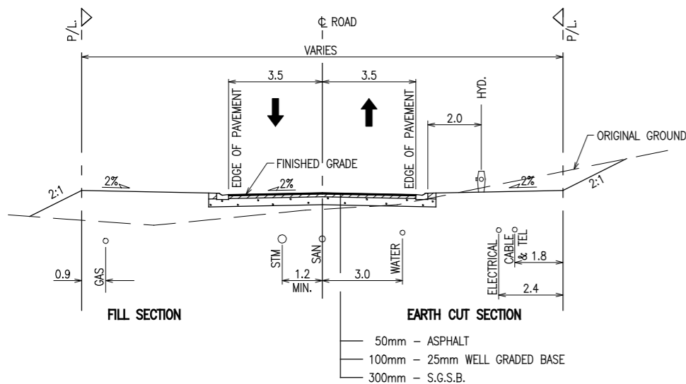
RESORT CORE TYPICAL SECTION
