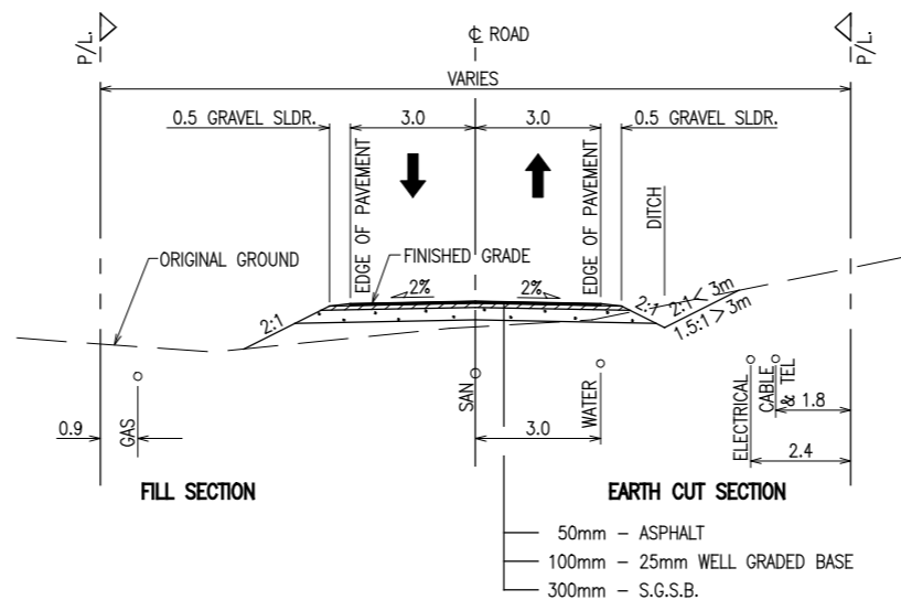
LOCAL ROAD TYPICAL SECTION
