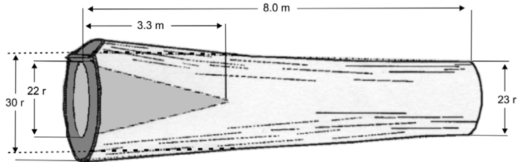
A log with simple butt rot estimated to penetrate 3.3 metres into the log (22 x 0.15 = 3.3m).
