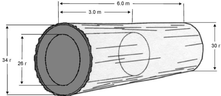
Figure 8.31 Ring Shake and Only the Core is Thick Enough to Produce Lumber.
