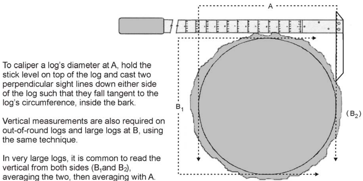
Figure 6.4 The Method of Measuring Butt Diameter by Callipering.
