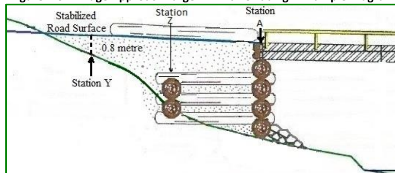
Figure 7-3 - Bridge Approach Large Fill with Cribbing – Example Diagram
