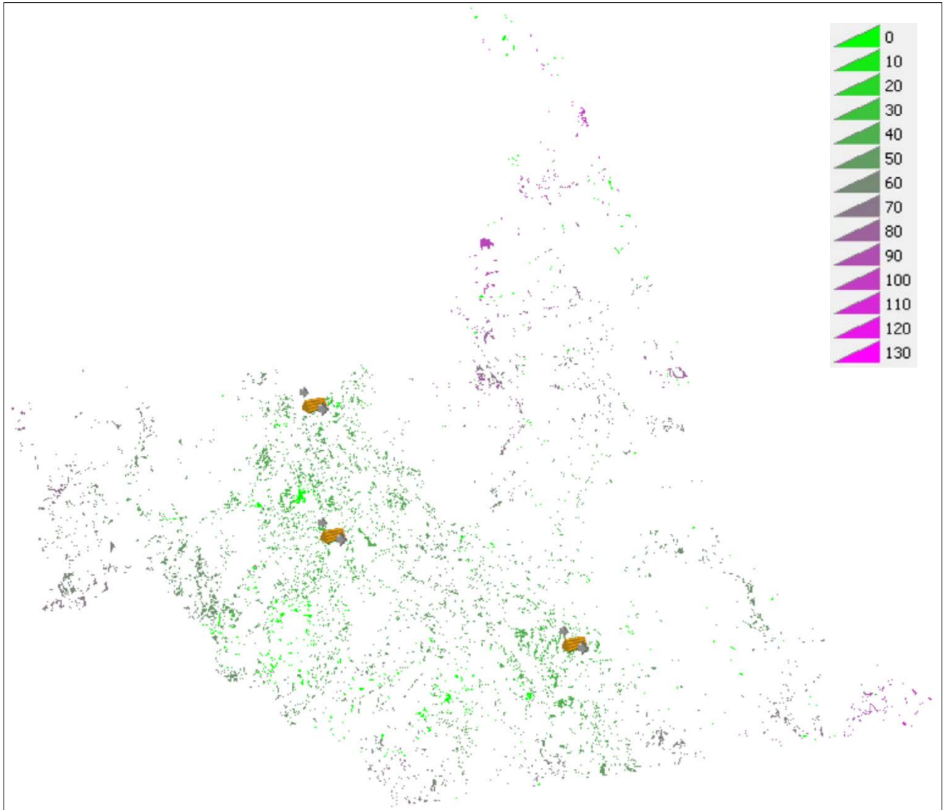
Figure 4. Spatial distribution of cutblocks by delivered biomass cost per odt (South).
