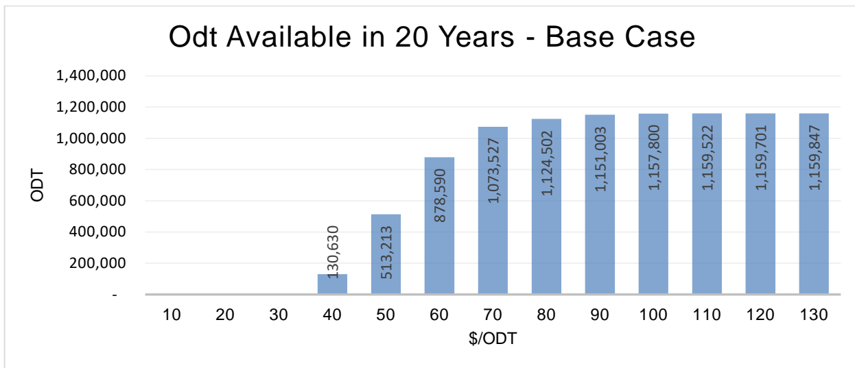
Figure 3. Cranbrook biomass 'cost-availability' in base case.
