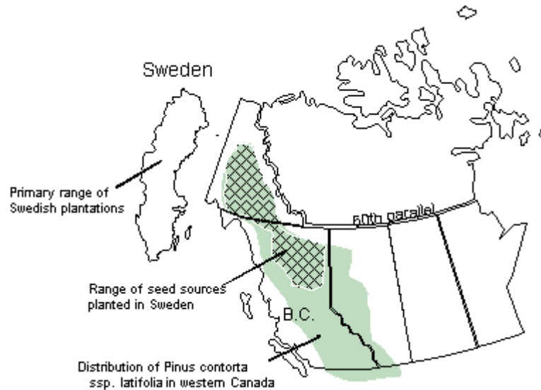
Figure 1. Distribution of Pinus contorta ssp. latifolia in Sweden and western Canada.
