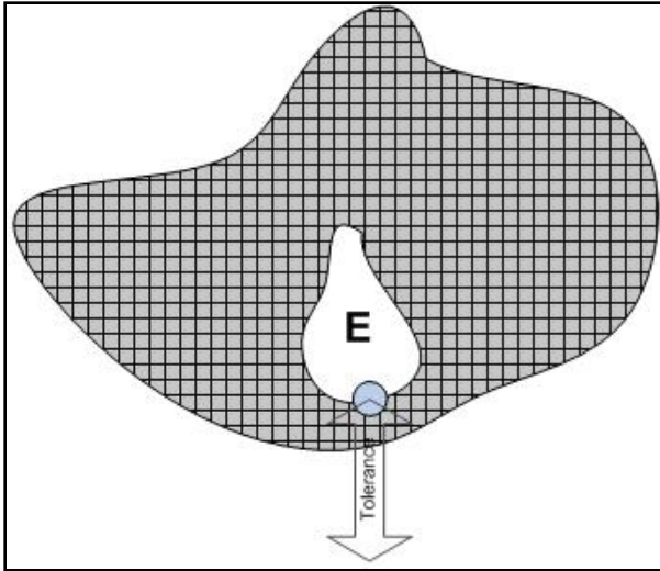
Figure 28. Self intersecting polygons.
