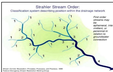
Figure 1. Diagram showing stream order of a watershed
