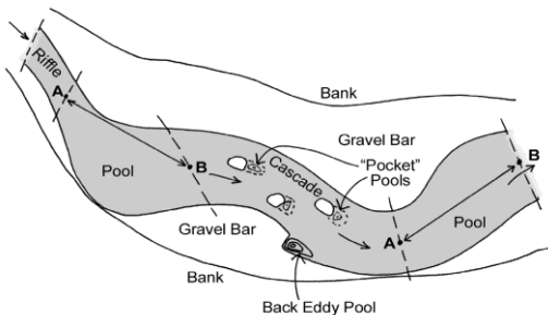
Figure 7. A plan-view sketch of two pool-riffle/cascade sequences in
