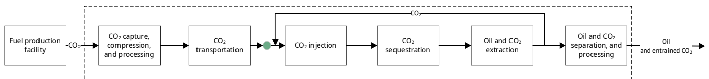
Figure 2: Project case – EOR- PFD
