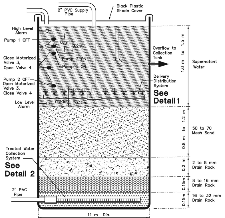
Figure 1 (a) Bio-Sand Filtration Tank
