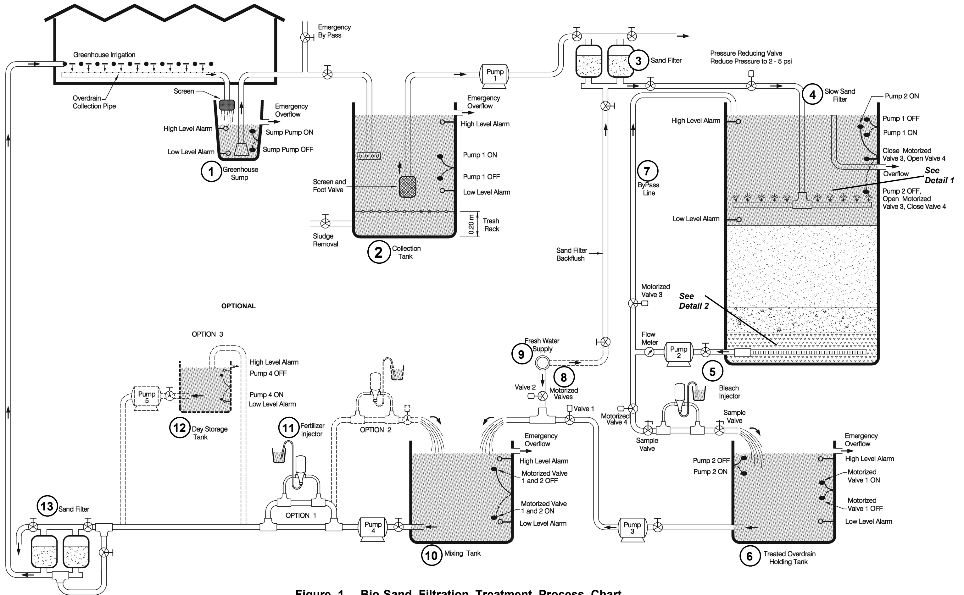
Figure 1 Bio-Sand Filtration Treatment Process Chart
