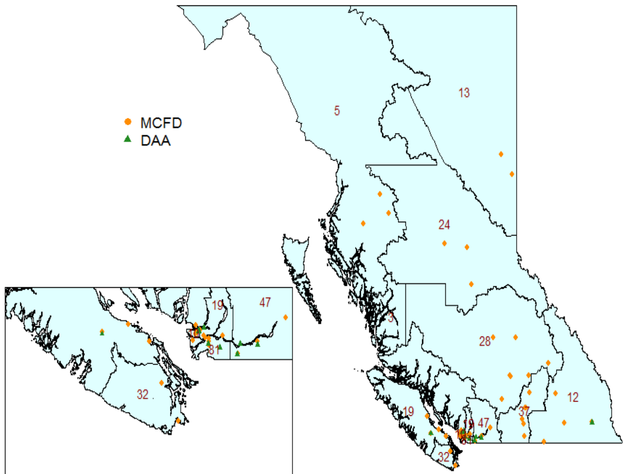
Figure 3: Number of Métis CCO by SDA and Office Location, as of July 2017
