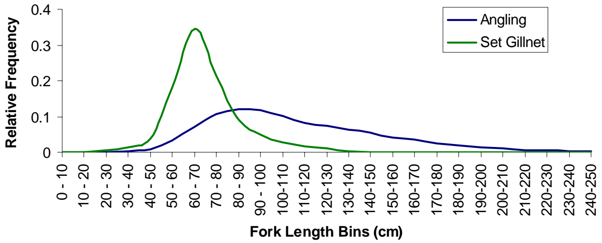
Figure 4. The relative size distribution of sturgeon caught in two gear types from six years of angling data and four years of Leq'aimel, Lakahahmen and Hatzic set gillnet data from the FRSCS First Nations stewardship database.
