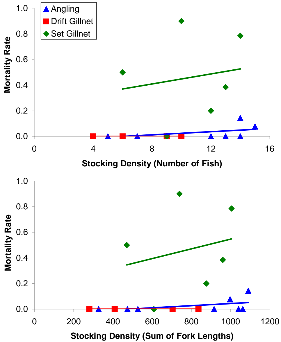
Figure 5. The relationship between mortality and stocking density for each gear type. Holding period was three days. Upper panel: Stocking density is the number of fish in each holding pen. Lower panel: Stocking density is the sum of the fork lengths of all the fish in each pen.
