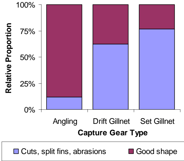
Figure 2. The relative proportions of sturgeon showing cuts, split fins or abrasions upon collection from three gear types, summer 2005. Note that major versus minor net-rashes and fin-splits were scored identically, thus differences between set and drift gillnet fish were less apparent in these analyses.
