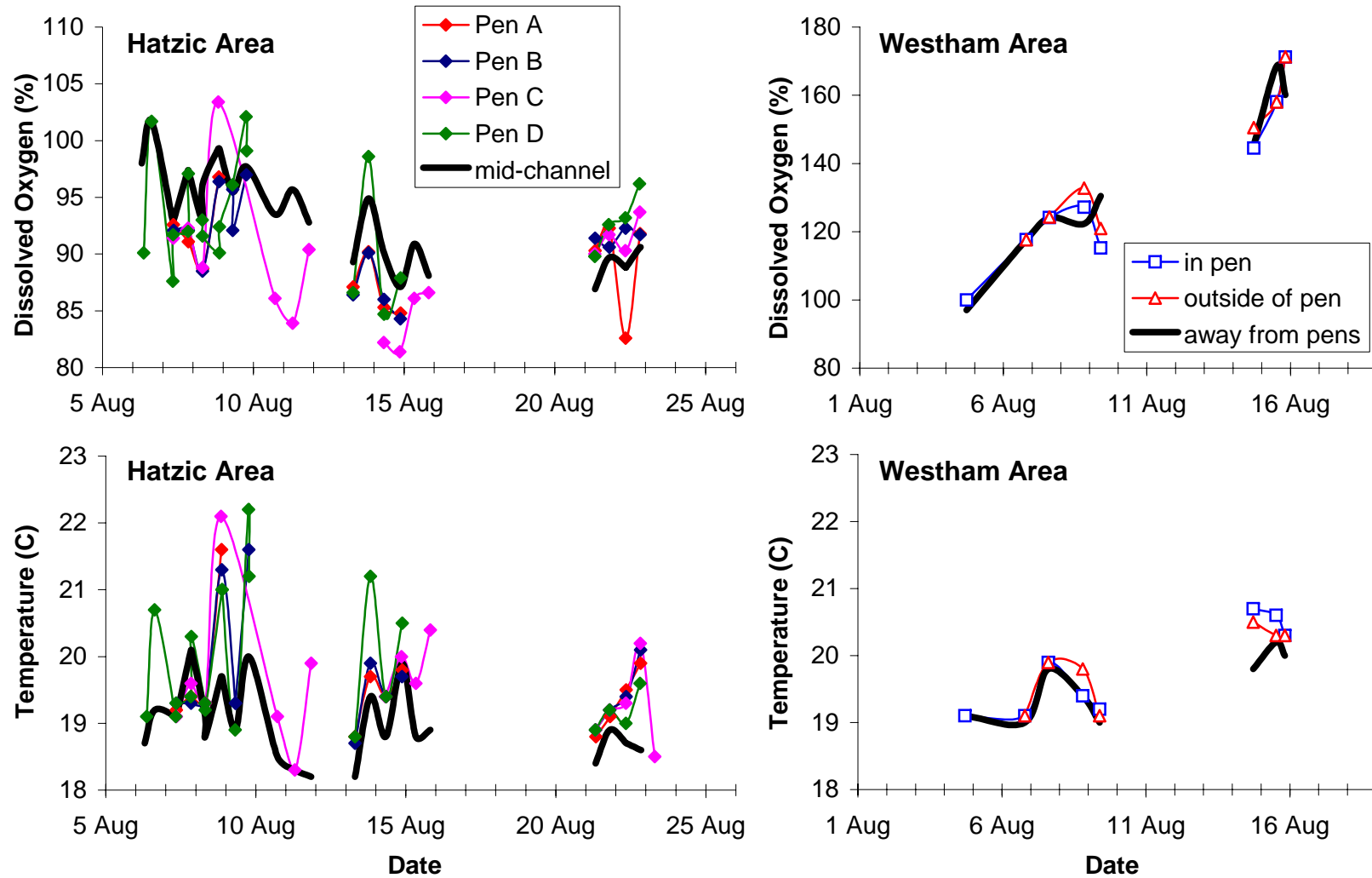
Appendix Figure A1. Dissolved oxygen and temperature of holding pens and of mid-channel surface water in the Hatzic Slough and Westham Island areas, 2005.
