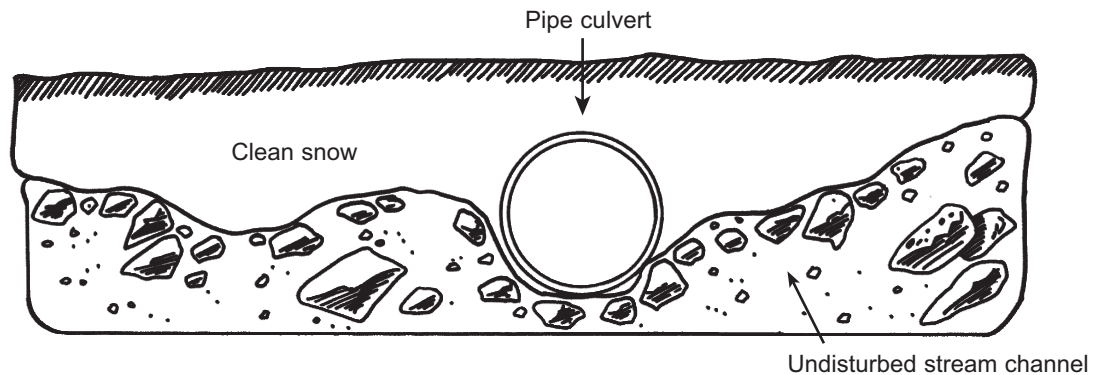
Figure 10. Temporary winter stream crossings using compacted snowfills. Culverts or heavy steel pipe allow meltwater to pass during warm weather trends.
