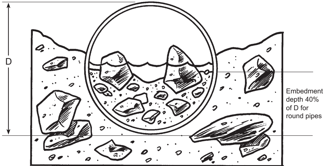
Culvert/streambed cross-section
