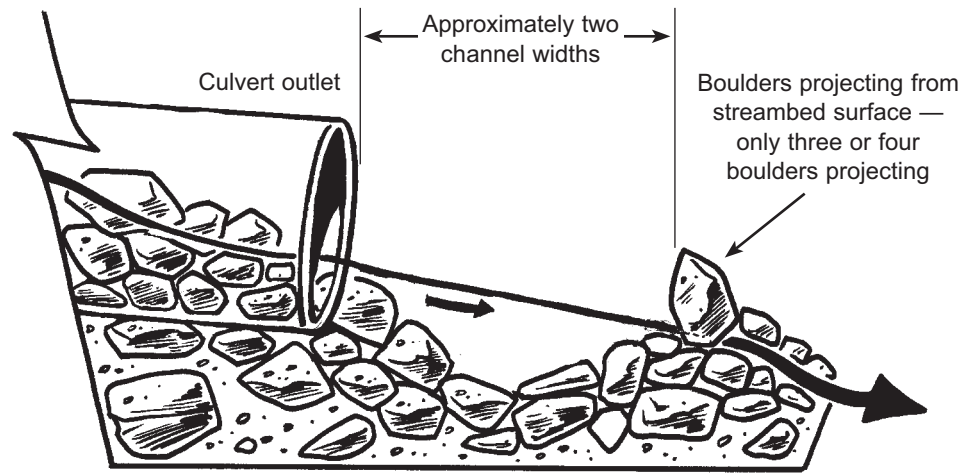
Figure 8. Typical downstream weir.
