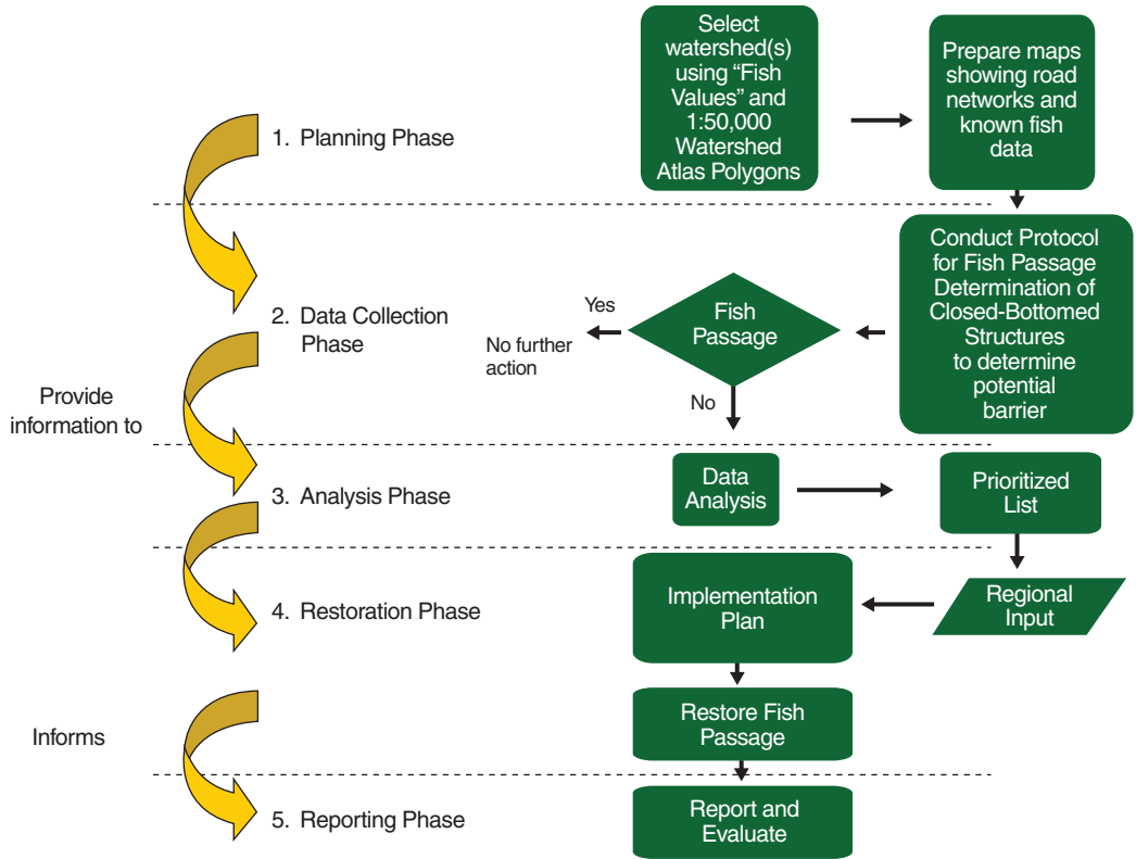
Figure 12. Overview of the five-phase provincial procedure for assessing and prioritizing the restoration of fish passage at culvert-stream crossings.
