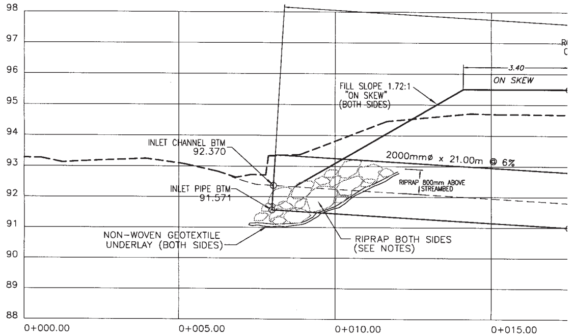
CULVERT (61'00" SKEW) SCALE HOR 1:10
