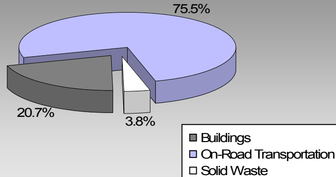
Fraser-Fort George Regional District Unincorporated Areas 2007 GHG Emissions Sources
