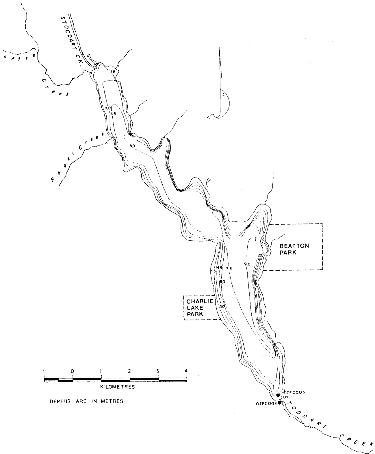
FIGURE 4 Charlie Lake Bathymetry
