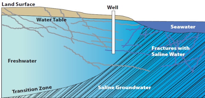
Figure 2: A fractured bedrock aquifer can deliver sea water to a well from a single fracture. (British Columbia , 2016)
