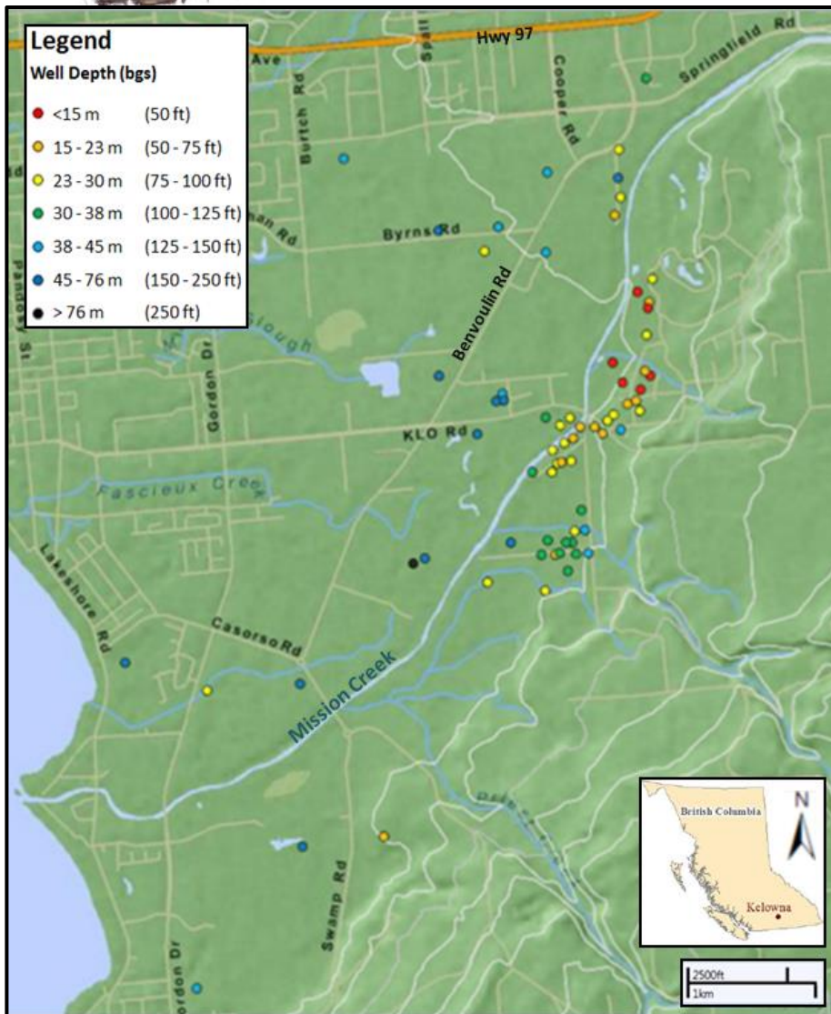
Figure 1: Flowing artesian wells in the Mission Creek area. (bgs: below ground surface)
