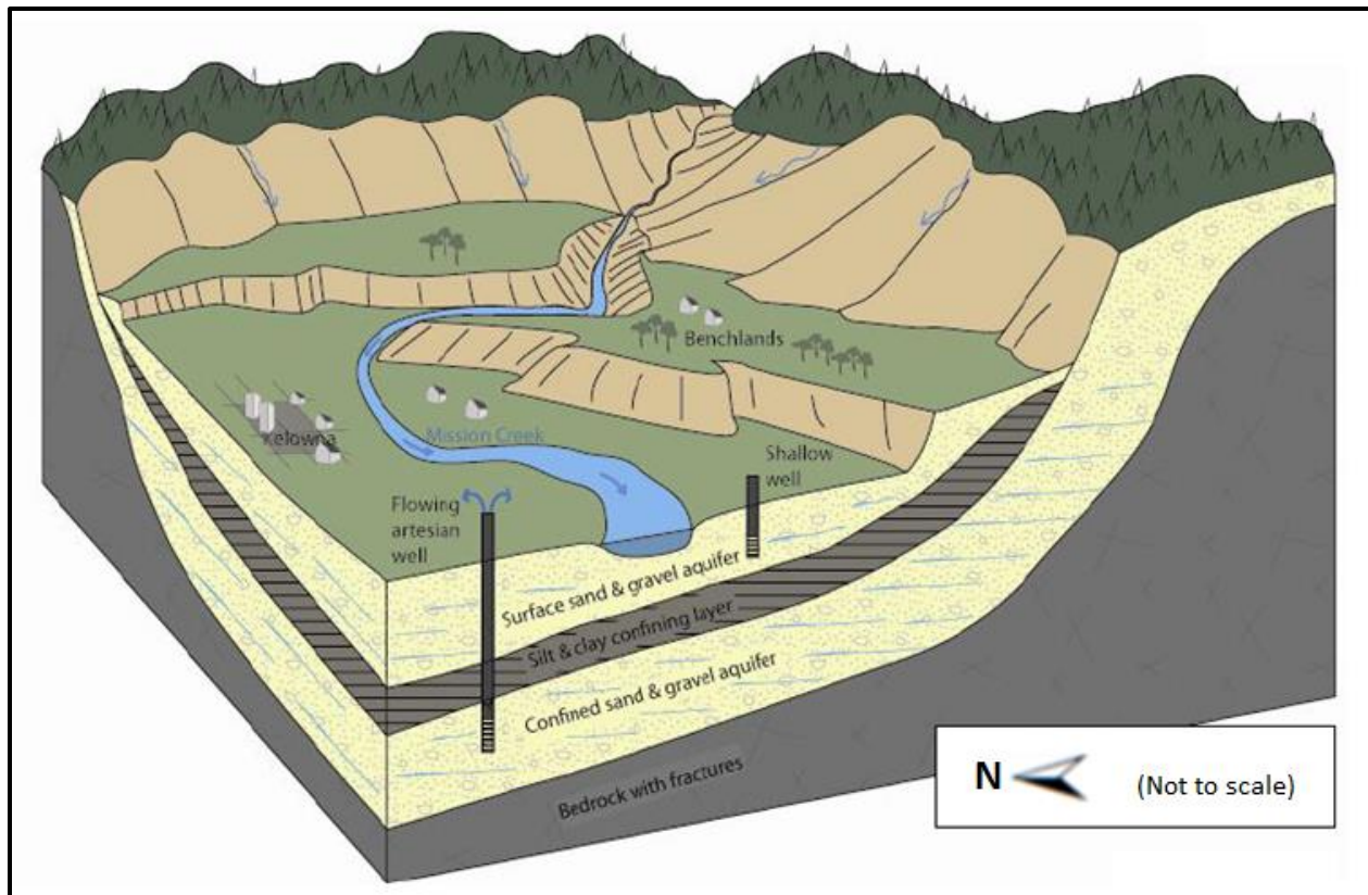
Figure 2: Simplified schematic of the Mission Creek aquifers
