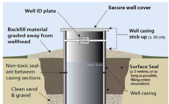
FIGURE 3 Properly constructed dug well
