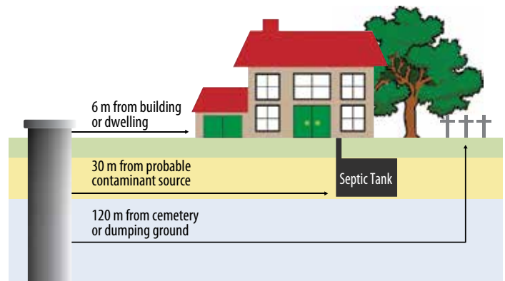
FIGURE 2 Regulated setbacks from potential contamination sources
