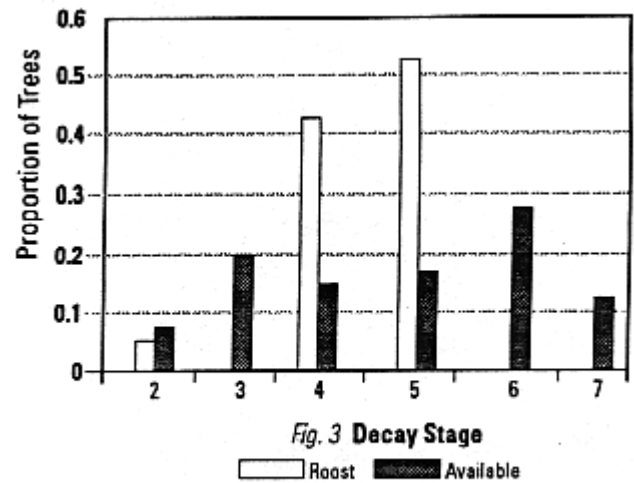
Figure 3. Roost trees by decay class.
