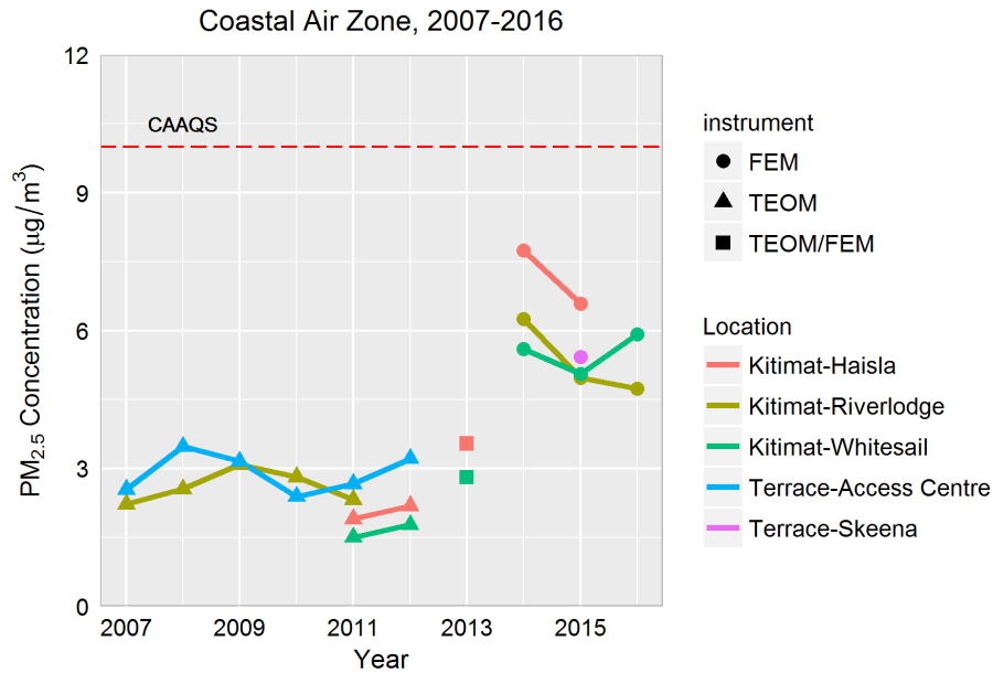
Figure 3. Trends in PM 2.5 concentrations (2007-2016), based on annual mean concentrations from a single year. The CAAQS value of 10 µg/m 3 is shown by the dashed line. PM 2.5 measurements prior to 2011 are reported at 25°C and 1 atm. From 2011 onward, measurements are reported at local conditions.
