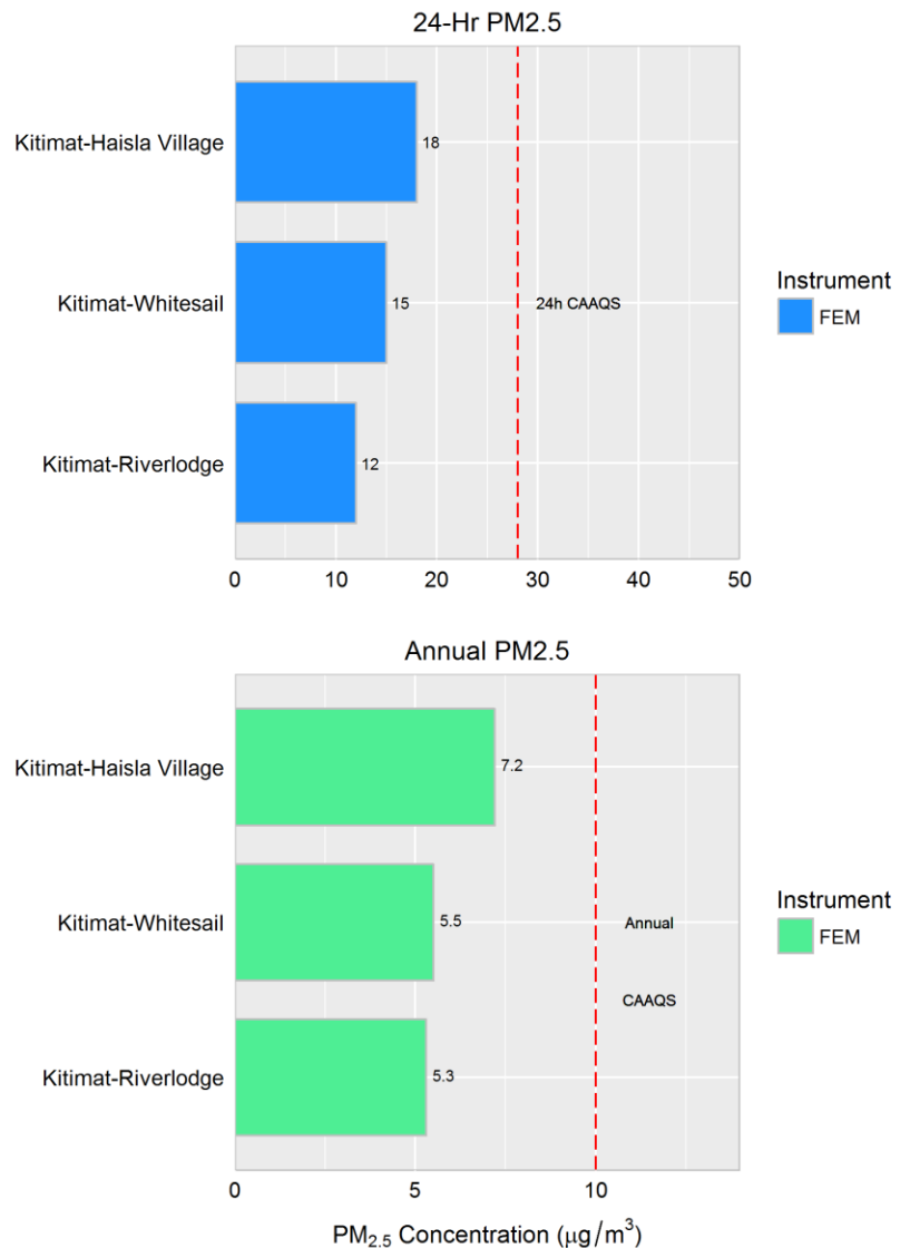
Figure 2. PM 2.5 concentrations in the Coastal Air Zone. Upper plot based on 24-hour concentration (annual 98 th percentile, averaged over 2014-2016). Lower plot based on annual mean concentration (averaged over 2014-2016). Red dashed lines identify CAAQS of 28 µg/m 3 (upper plot) and 10 µg/m 3 (lower plot).
