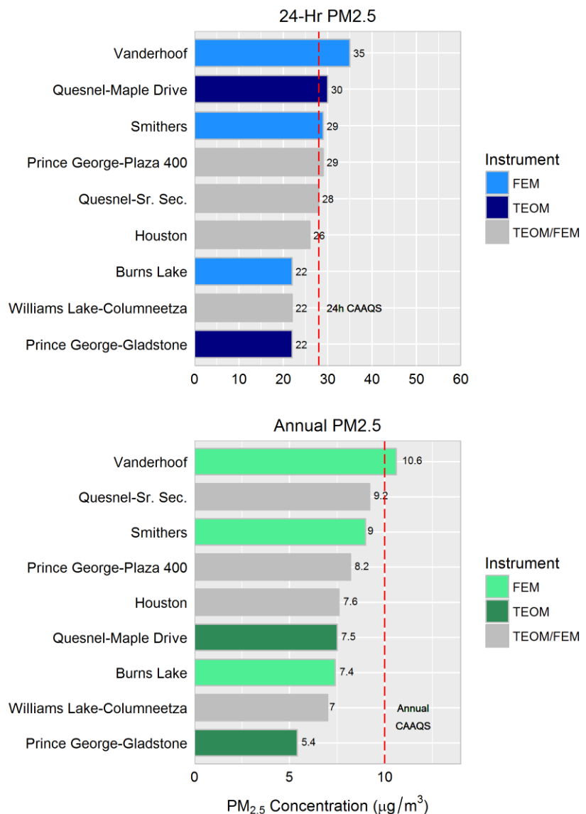
Figure 4. PM 2.5 concentrations in Central Interior Air Zone. Upper plot based on 24-hour concentration (annual 98 th percentile, averaged over 2013-2015). Lower plot based on annual mean concentration (averaged over 2013-2015). The red dashed lines identify CAAQS of 28 µg/m 3 (upper plot) and 10 µg/m 3 (lower plot).
