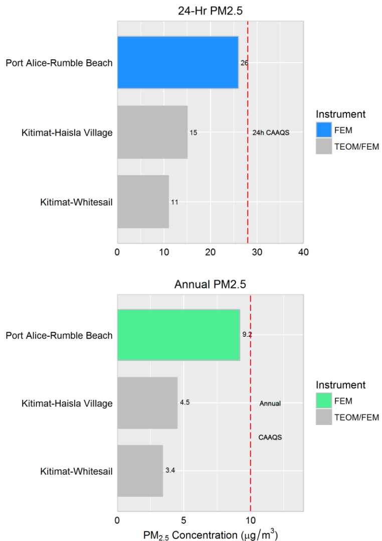
Figure 2. PM 2.5 concentrations in Coastal Air Zone. Upper plot based on 24-hour concentration (annual 98 th percentile, averaged over 2012-2014). Lower plot based on annual mean concentration (averaged over 2012-2014). Red dashed lines identify CAAQS of 28 µg/m 3 (upper plot) and 10 µg/m 3 (lower plot).
