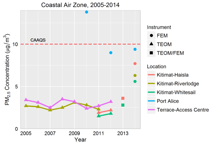
Figure 3. Trends in PM 2.5 concentrations (2005-2014), based on annual mean concentrations from a single year. The CAAQS value of 10 µg/m 3 is shown by the dashed line. PM 2.5 measurements prior to 2011 are reported at 25°C and 1 atm. From 2011 onward, measurements are reported at local conditions.
