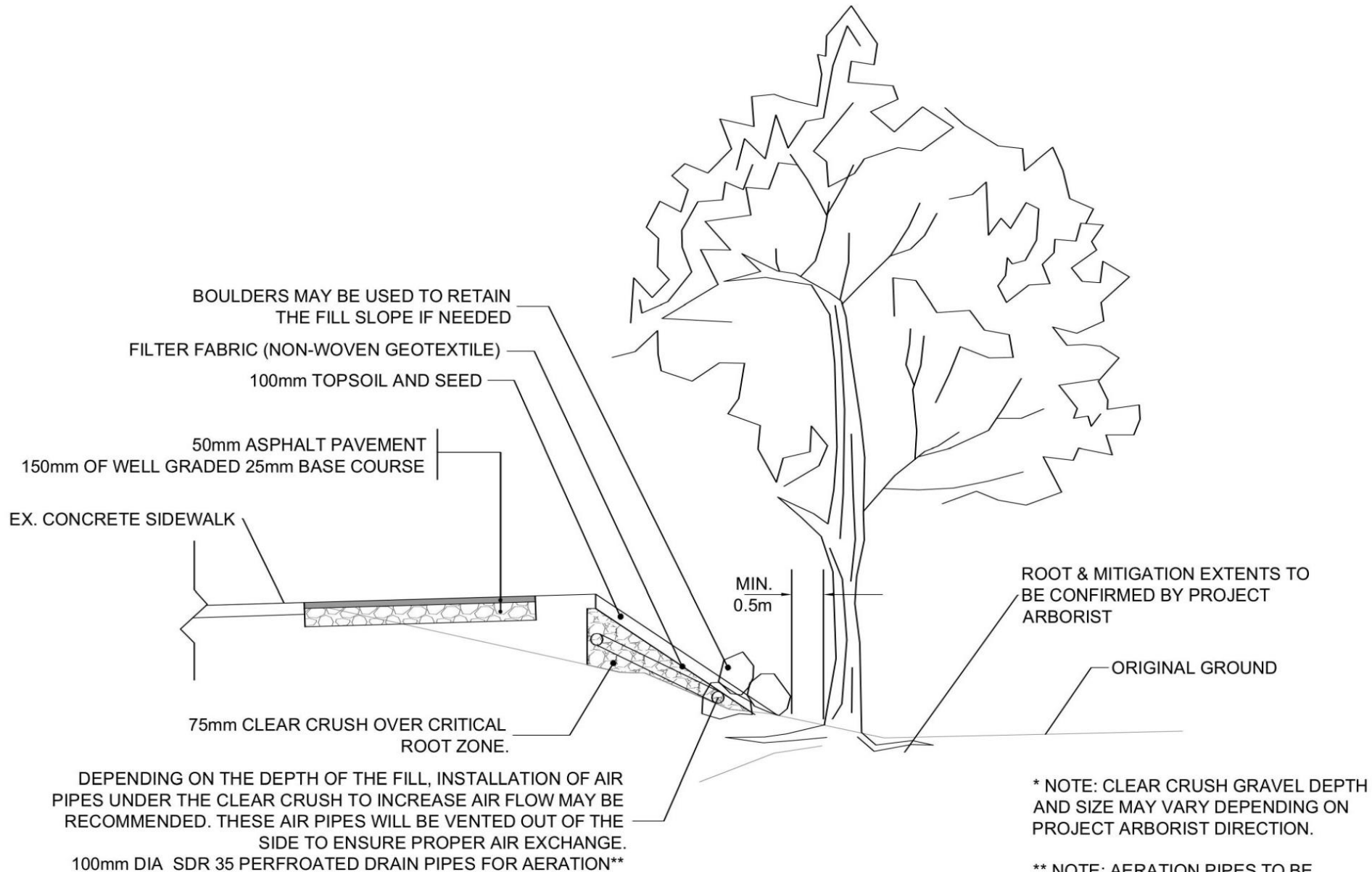
TREE ROOT MITIGATION DETAIL ON FILL SLOPES
