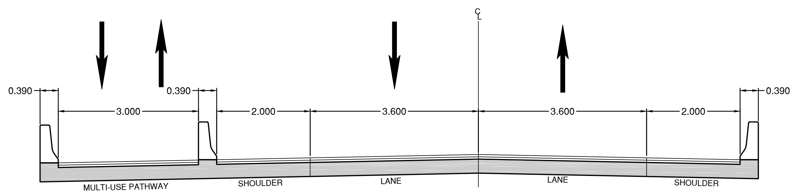
LIZARD CREEK BRIDGE TYPICAL CROSS SECTION
