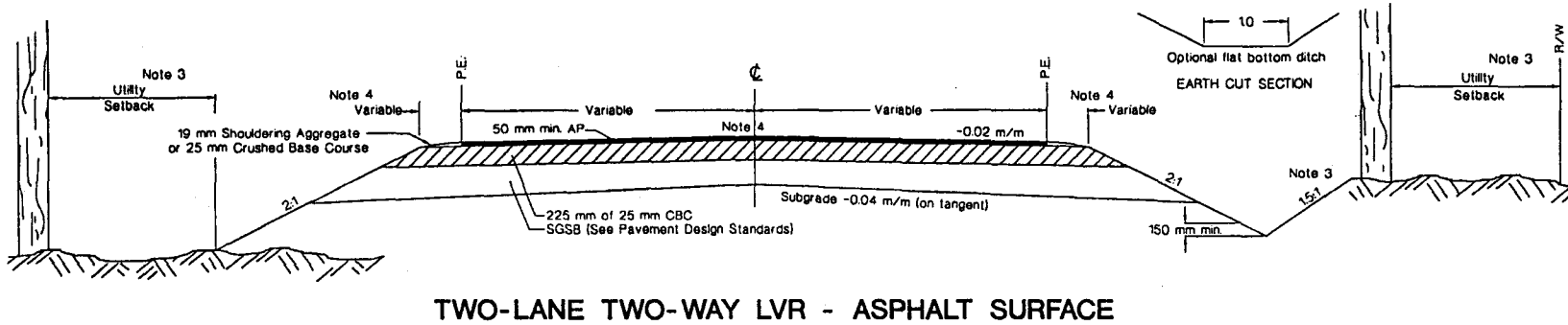
Figure 510.0 Cross Section for Low-Volume Roads
