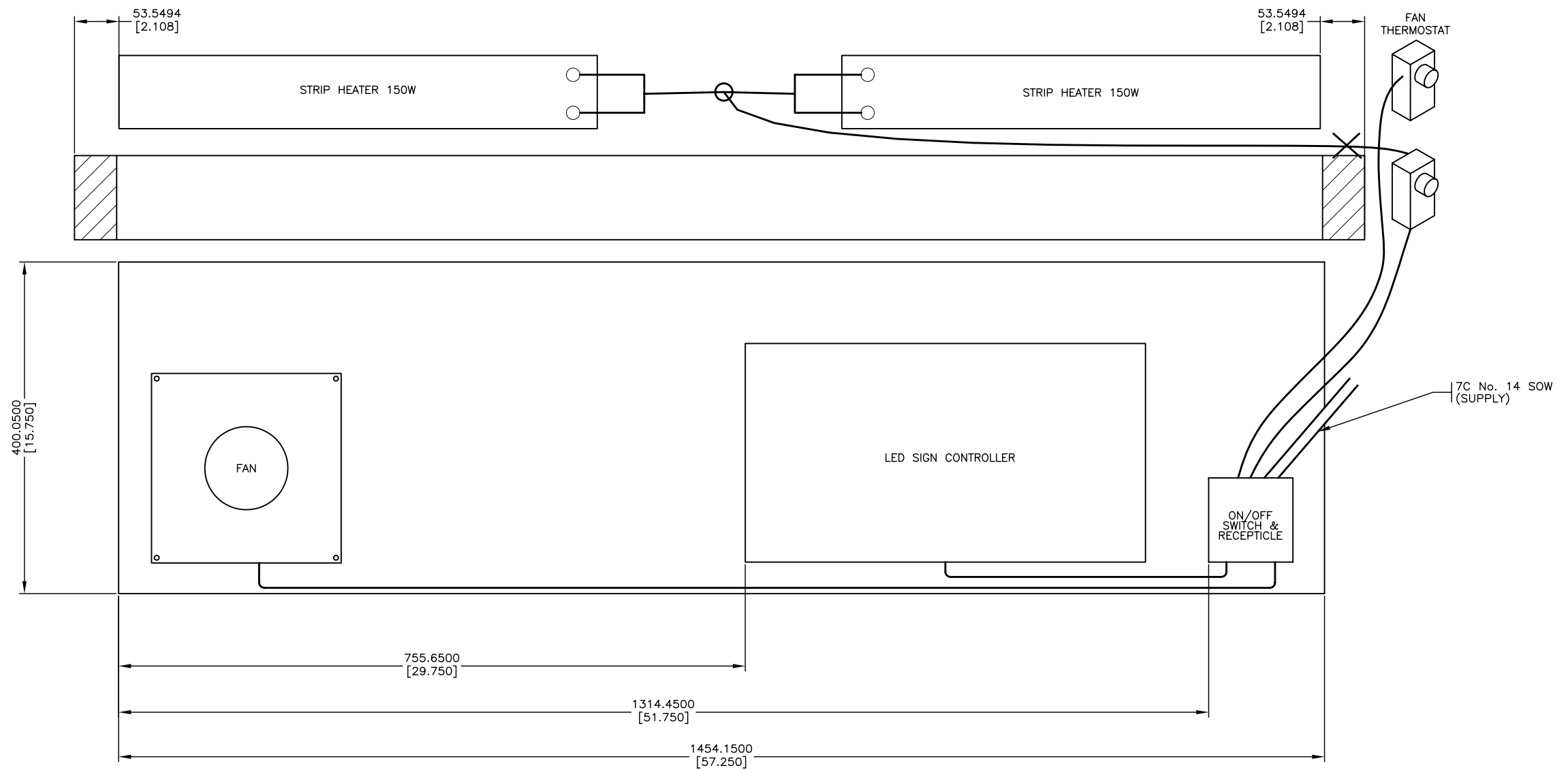
COMPONENT BOARD 1:3
