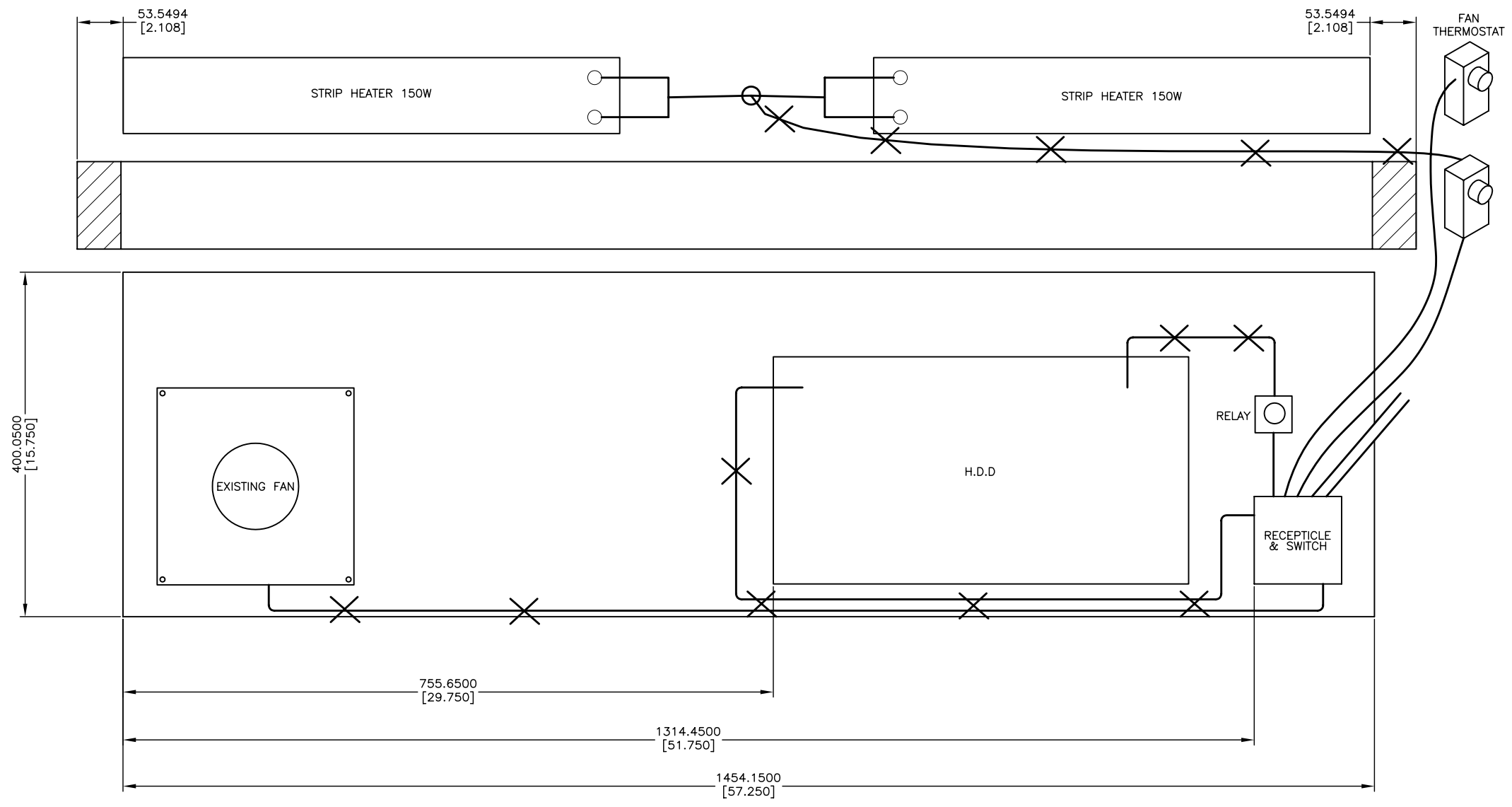
COMPONENT BOARD 1:3
