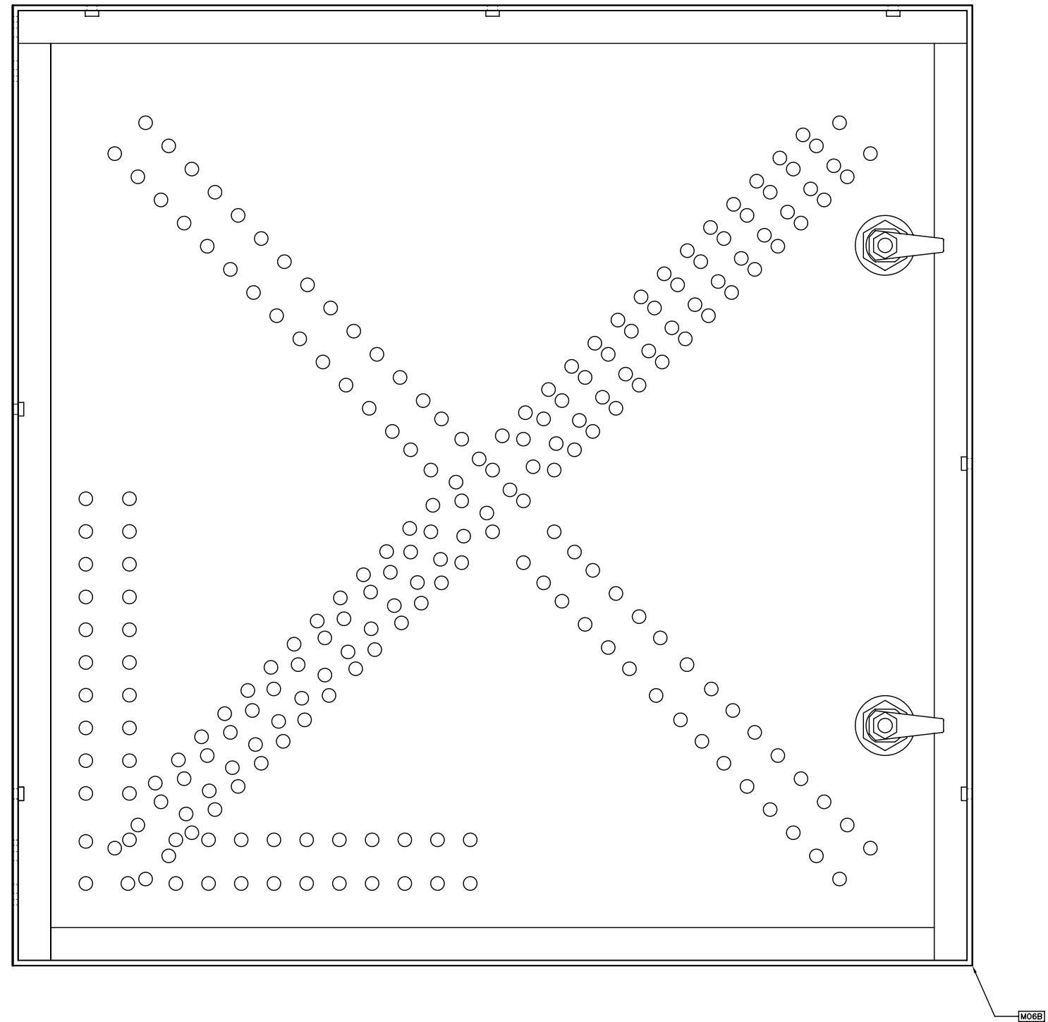
DOOR SUB-ASSEMBLY (2 COLOUR) – BACK VIEW
