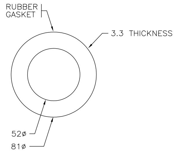
RUBBER GASKET DETAIL
