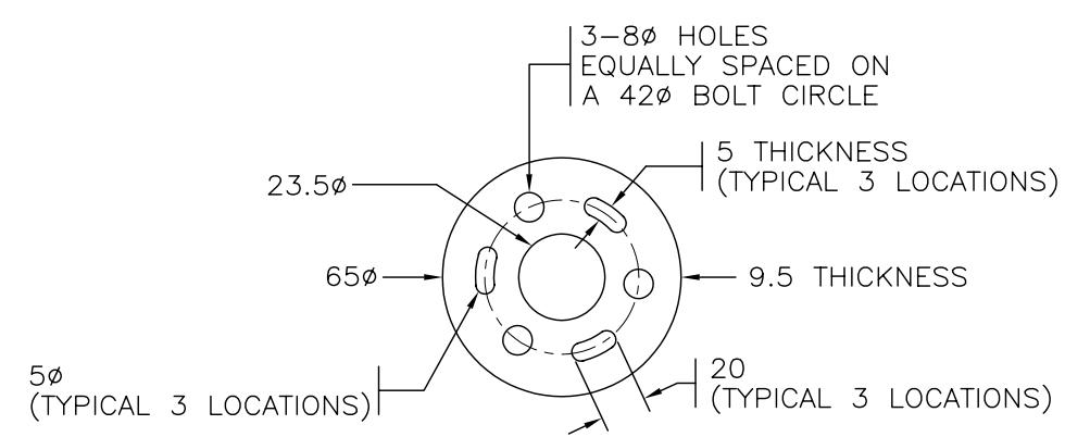
CAST ALUMINUM WASHER DETAIL
