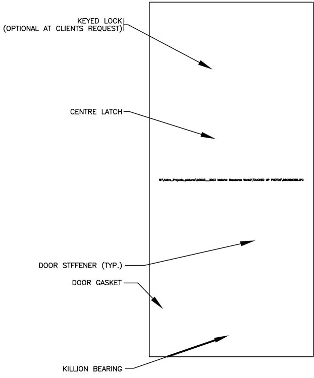
FIGURE 2 3 POINT LATCH 410.4
