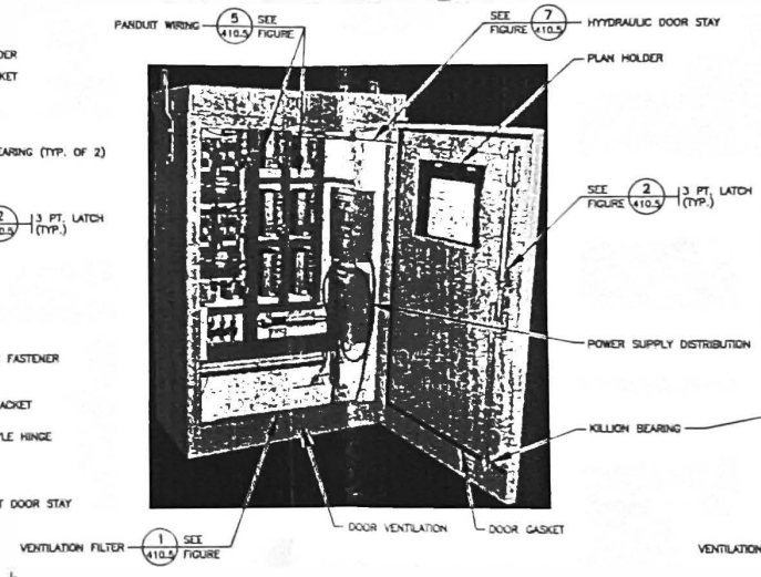
FIGURE 4 SINGLE DOOR KIOSK - OPEN 410.2
