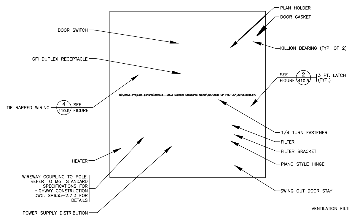
FIGURE 2 POLE MOUNT CABINET – OPEN 410.3
