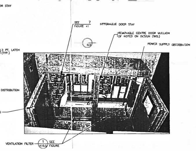
FIGURE 6 DUAL DOOR KIOSK OPEN 410.1
