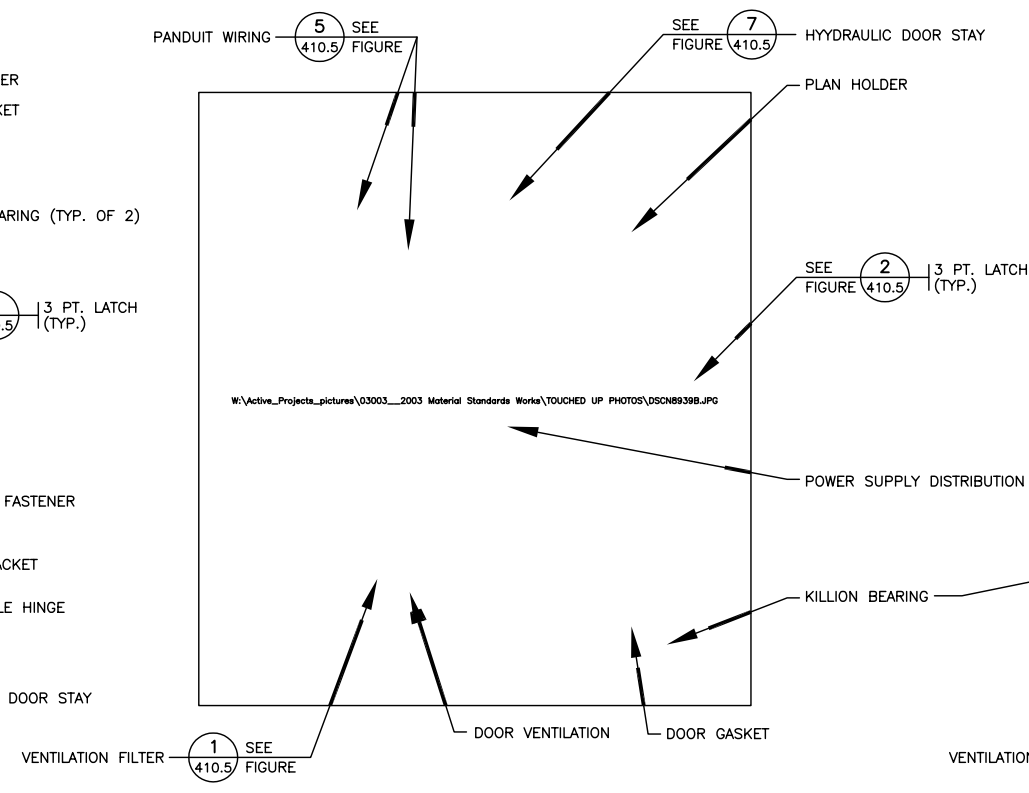
FIGURE 4 SINGLE DOOR KIOSK – OPEN 410.2
