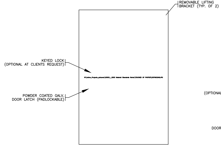
FIGURE 3 SINGLE DOOR KIOSK – CLOSED 410.2
