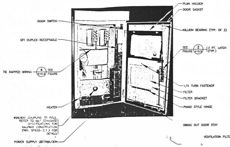
FIGURE 2 POLE MOUNT CABINET OPEN 410.3
