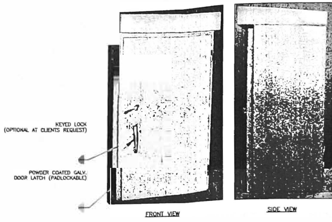
FIGURE 1 POLE MOUNT CABINET CLOSED 410.3
