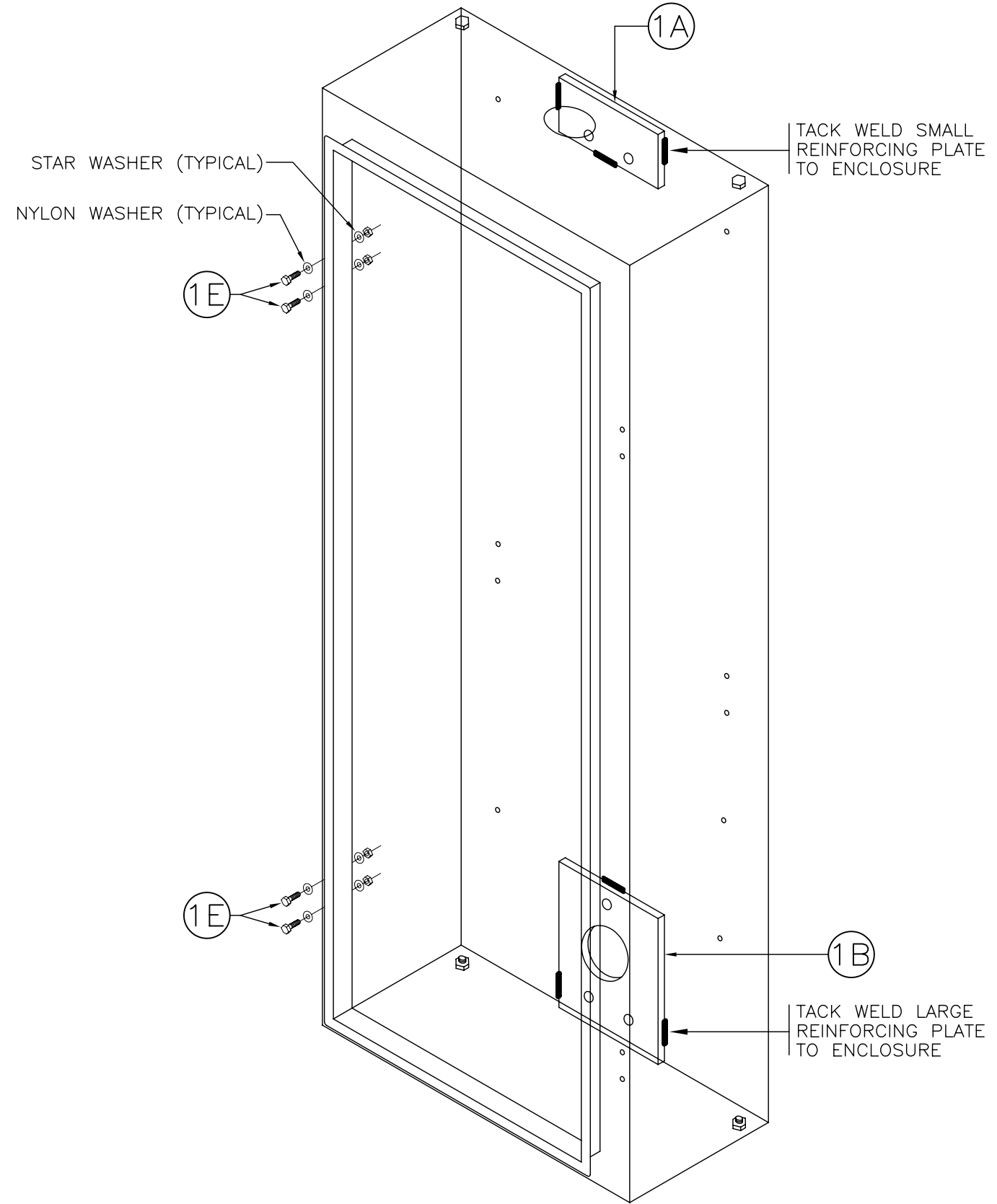
ASSEMBLY VIEW
