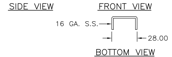
ITEM 12B (DOOR LOCK RAIL)
