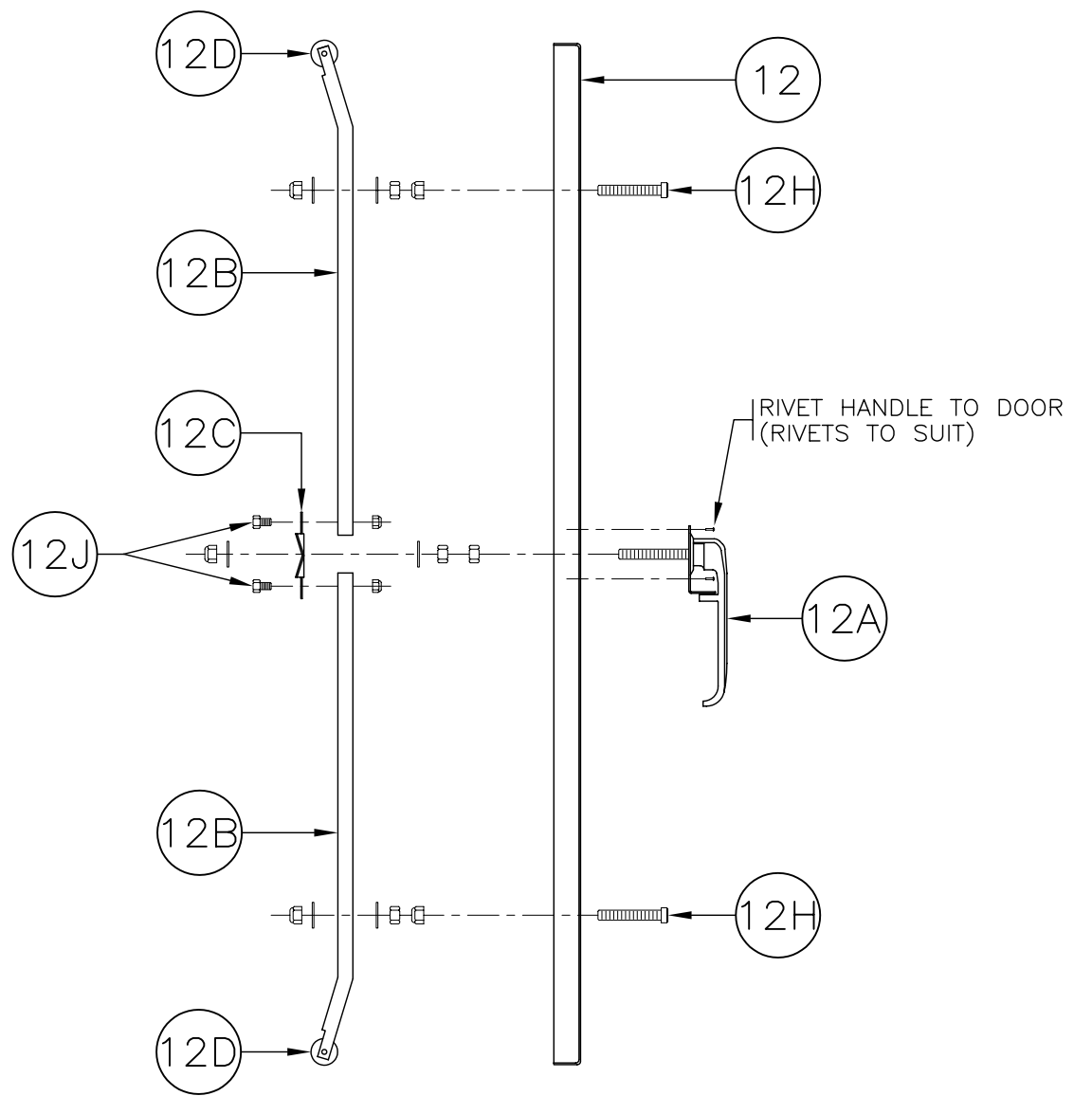
SIDE VIEW
