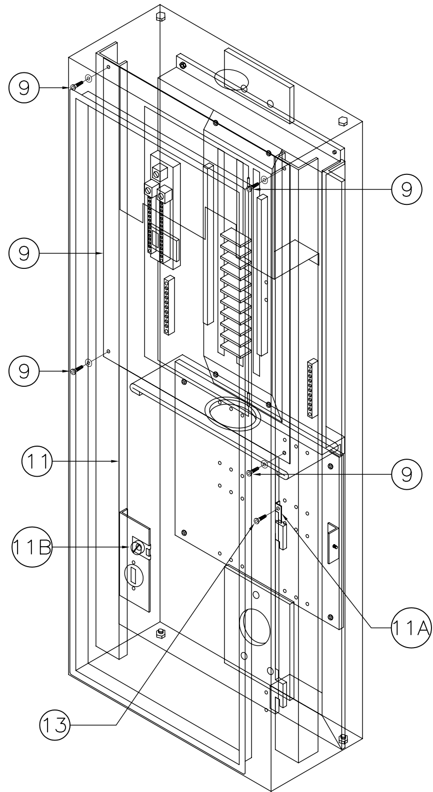
ASSEMBLY VIEW
