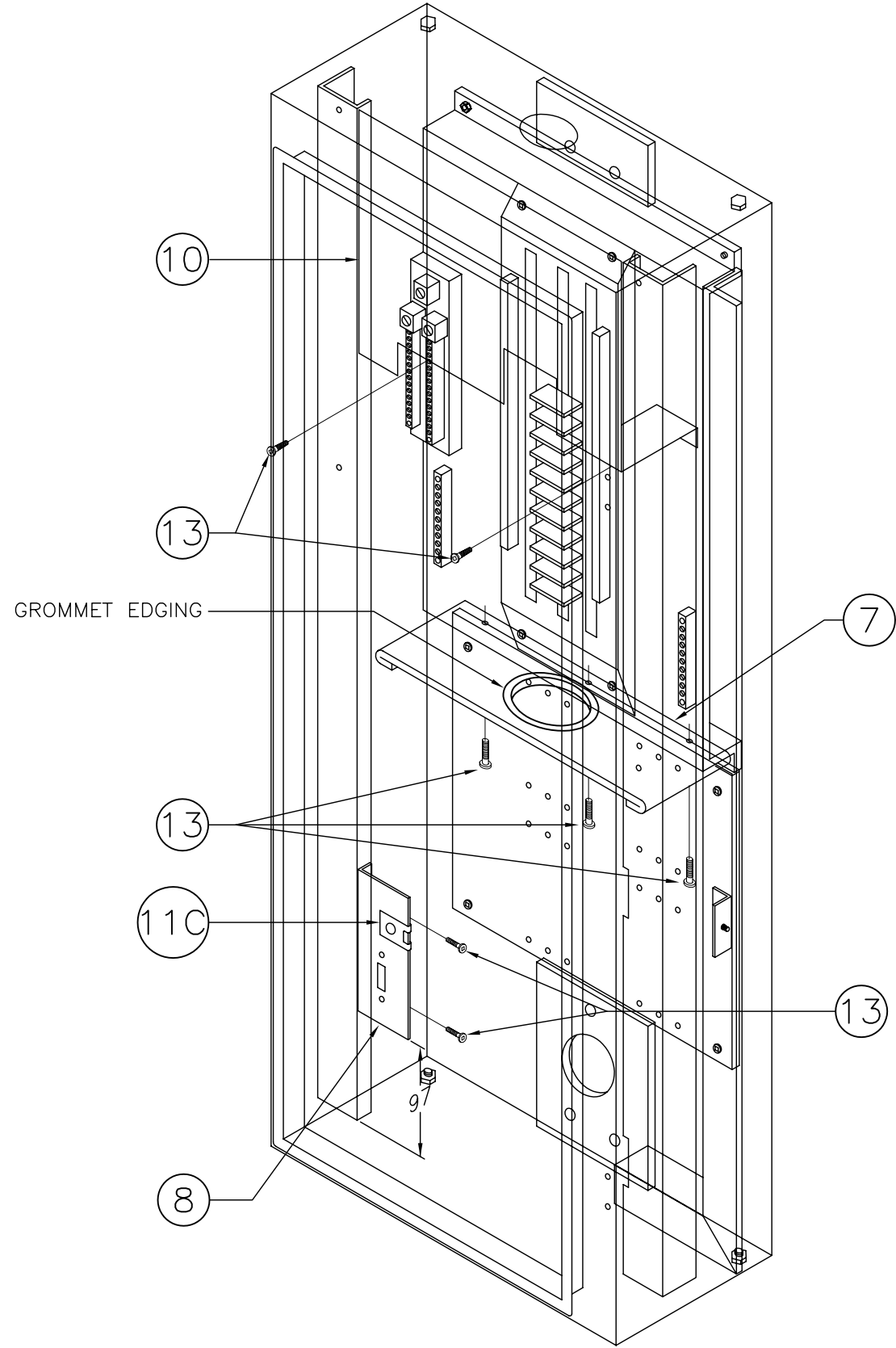
ASSEMBLY VIEW
