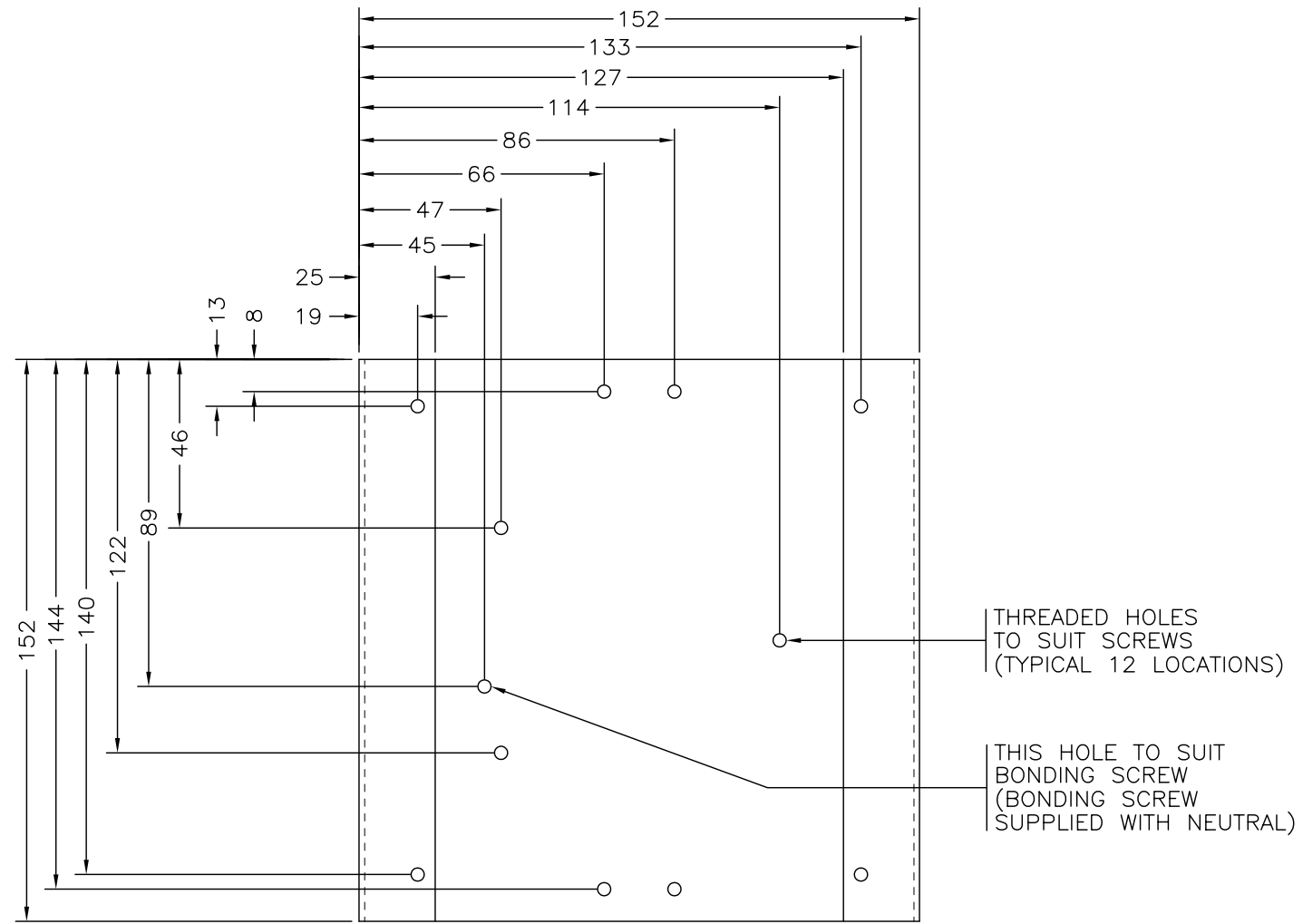
FRONT VIEW
