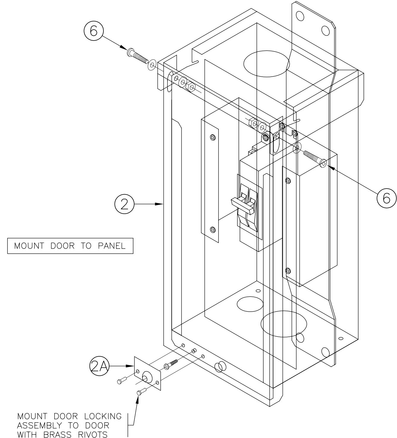
ASSEMBLY VIEW
