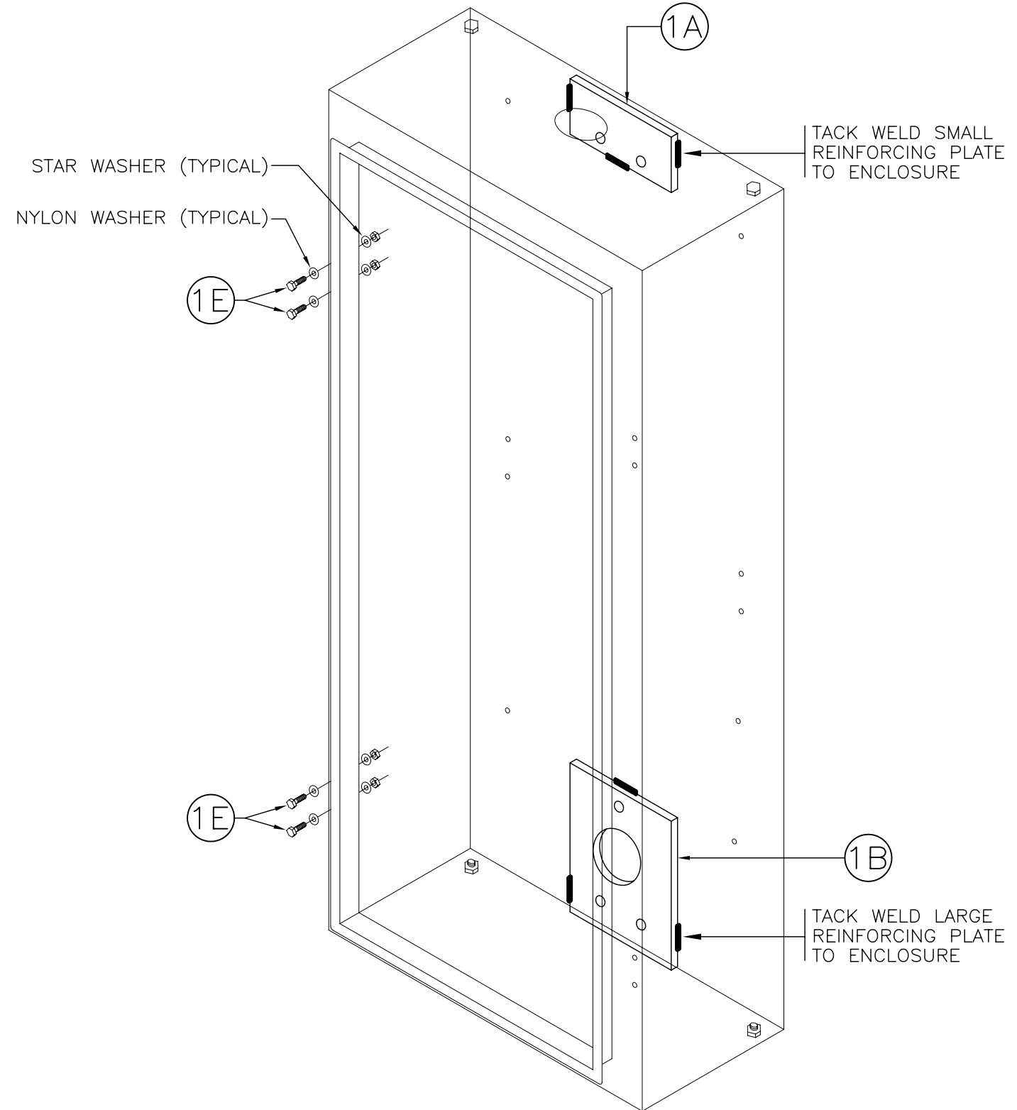
ASSEMBLY VIEW
