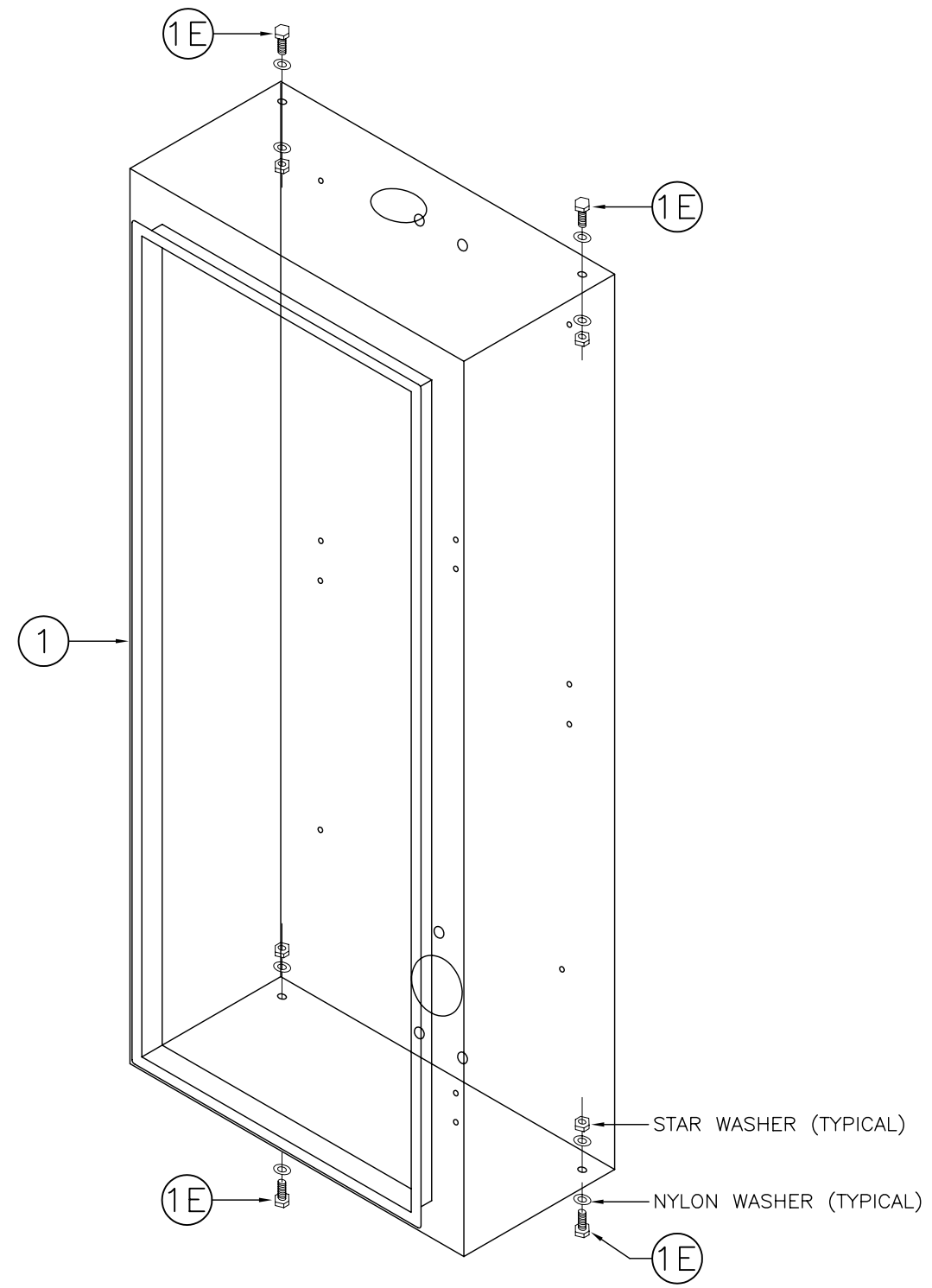
ASSEMBLY VIEW
