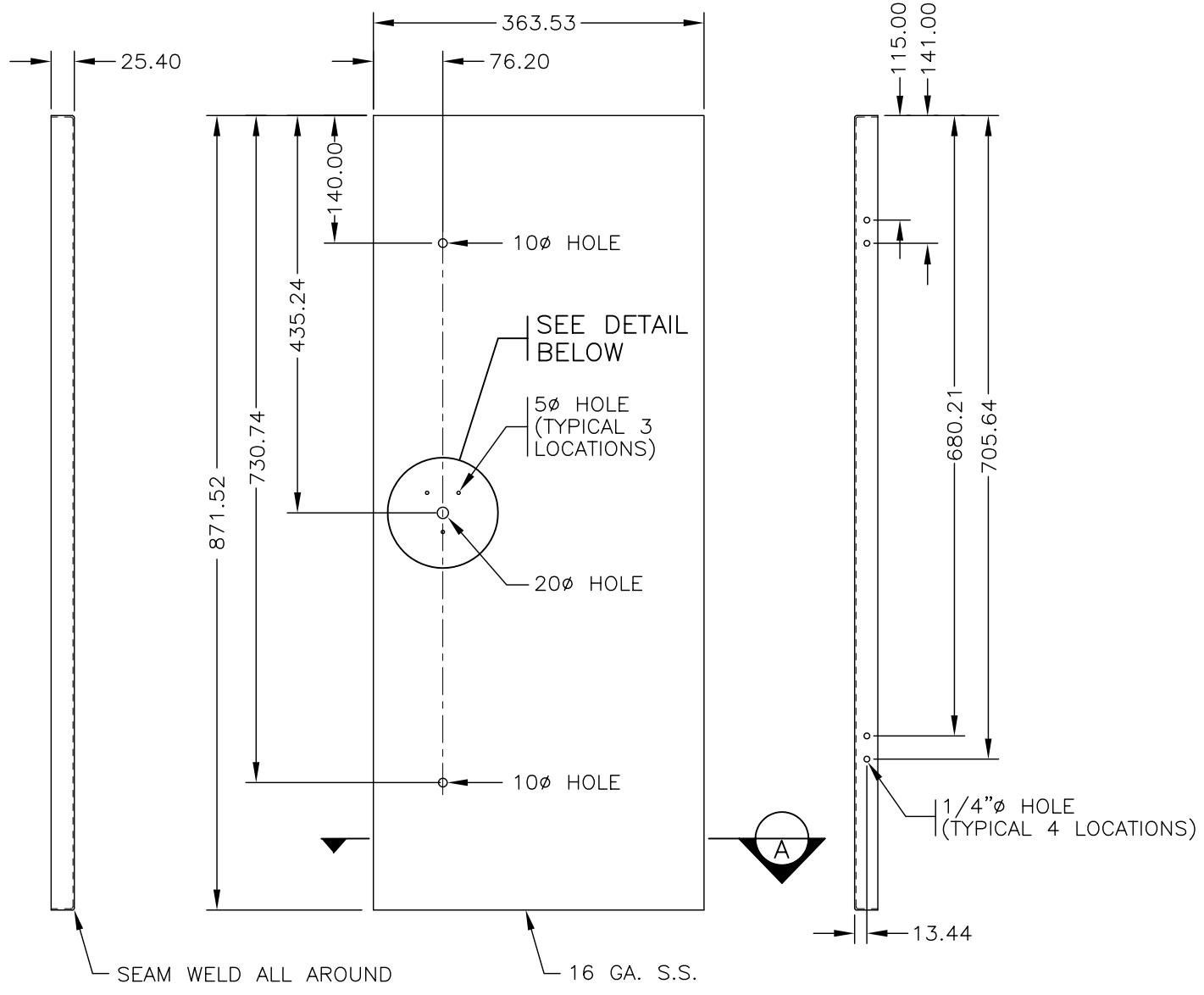
SIDE VIEW
