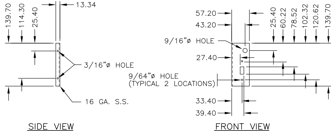
ITEM 9 (BYPASS SWITCH MOUNTING PLATE)
