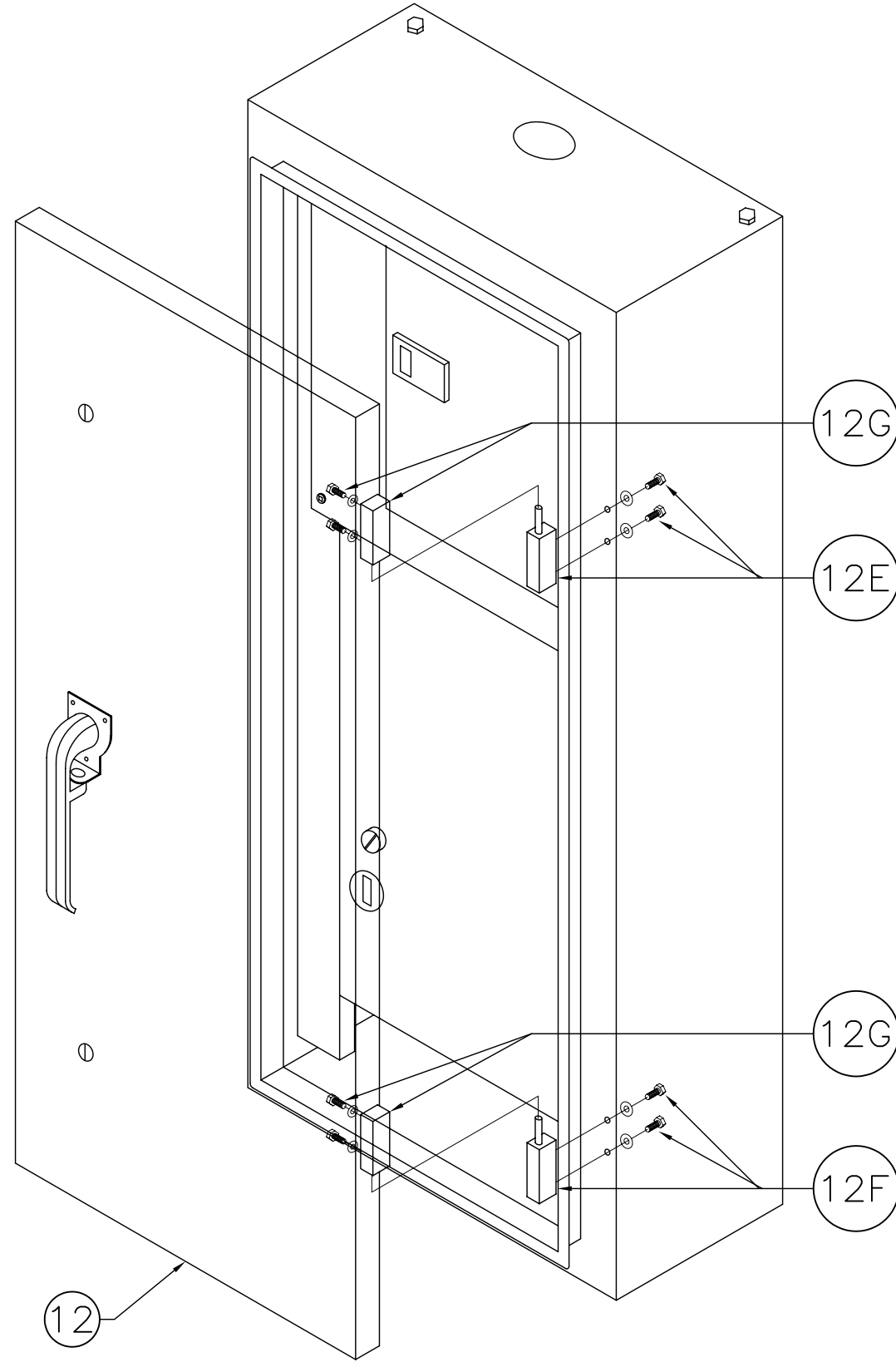
ASSEMBLY VIEW
